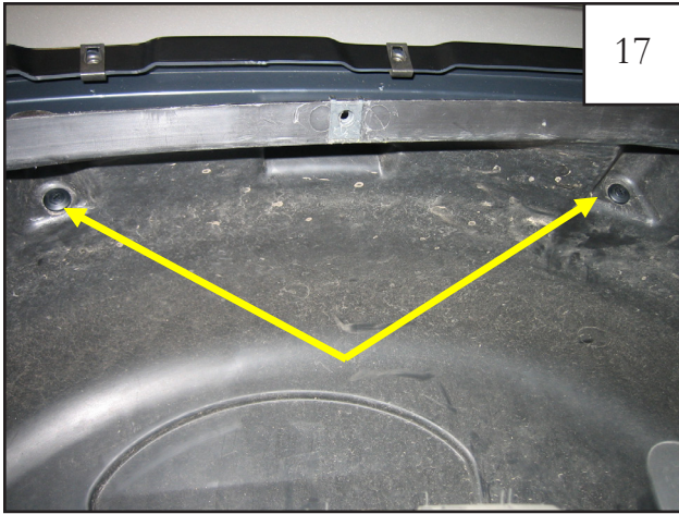
17 Position splash shield in wheel well, and install two supplied Plastic Phillips Head Tuflocs in upper pockets using a pushing-twisting motion.
